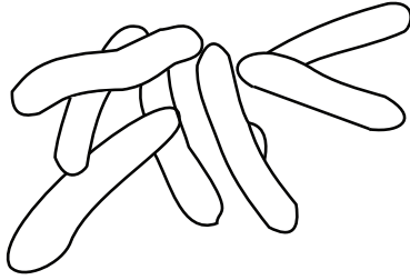
Mycobacterium leprae
