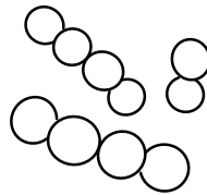
Lactococcus
